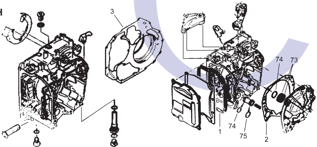
Transmission Casing
